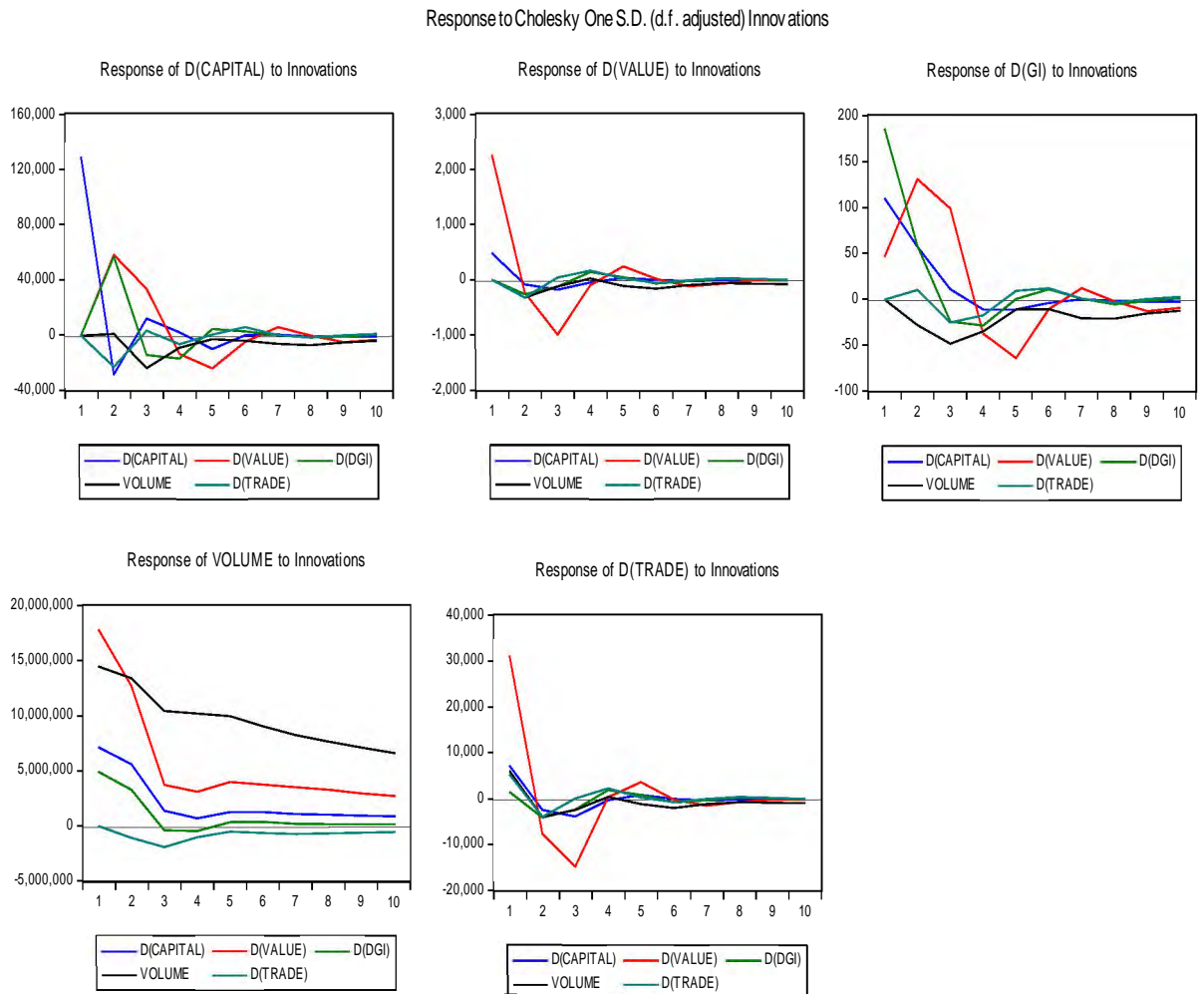
Figure 4.19: The combined graph of the impulse responses of the estimated VAR(2) model
