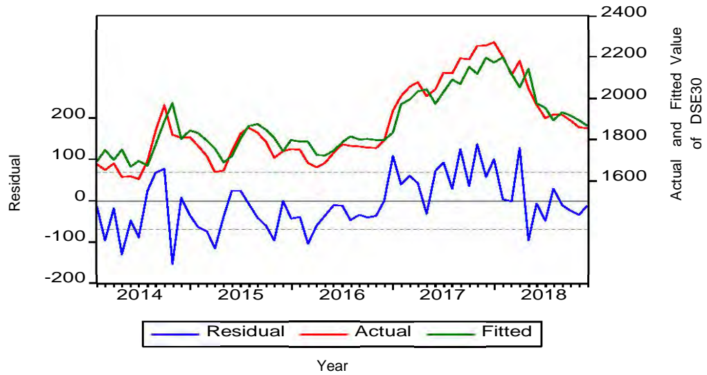
Figure 4.31: Actual, fitted, and residual plot of ARIMA(1,0,1) model of DSE30
