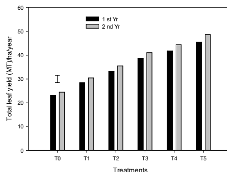
Figure 12.8: Total leaf yield/ha/year of mulberry as influenced by various levels of N management practices. Where, T 0 = 0 kg N/ha/yr, T 1 = 80 kg N/ha/yr, T 2 = 160 kg N/ha/yr, T 3 = 240 kg N/ha/yr, T 4 = 320 kg N/ha/yr and T 5 = 400 kg N/ha/yr. Vertical bar represent LSD ( P = 0.105 ) different levels of nitrogen and mulberry plant age interactions.
