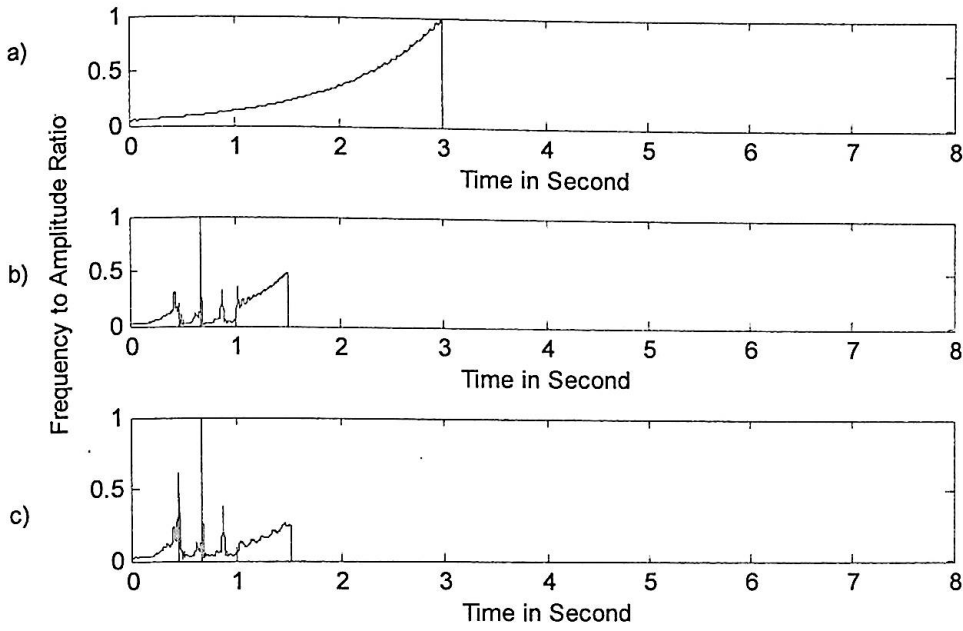
Fig. 4.14 Time frequency to amplitude analysis of synthetic earthquake wave respectively of Fig. 4.1.
