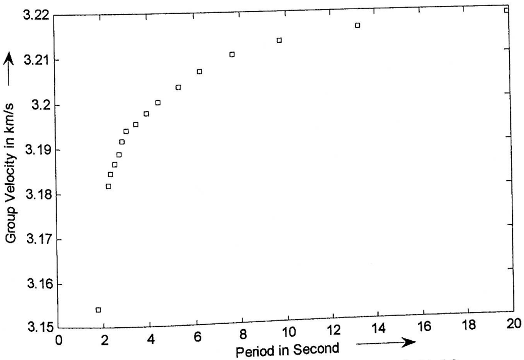
Fig. 5.5 Dispersion curve using the model parameters of table 5.2
