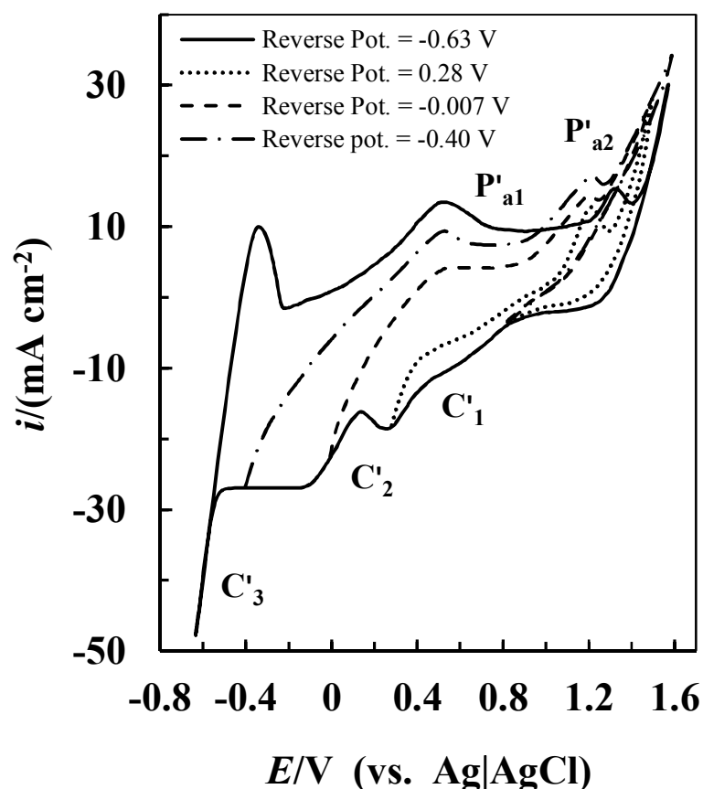
Figure 5.28 Effect of sweeping potential on the cyclic voltammograms recorded on a pellet of waste lead, graphite and paraffin mixture electrode in 1\ mol\ dm^{-3}\ HNO_3 at 30^\circ\ C with a scan rate of 10\ mV\ s^{-1} .
