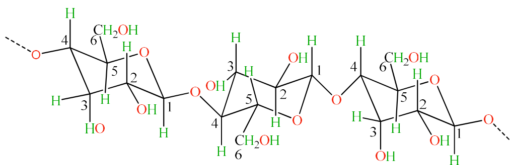
Scheme 1.2: Rod like chain structure of cellulose
