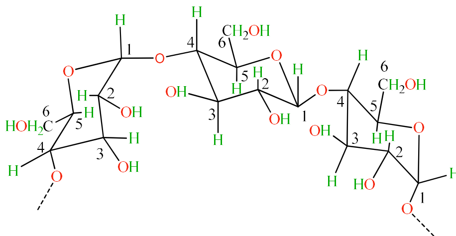
Scheme 1.3: Helix like chain structure of starch
