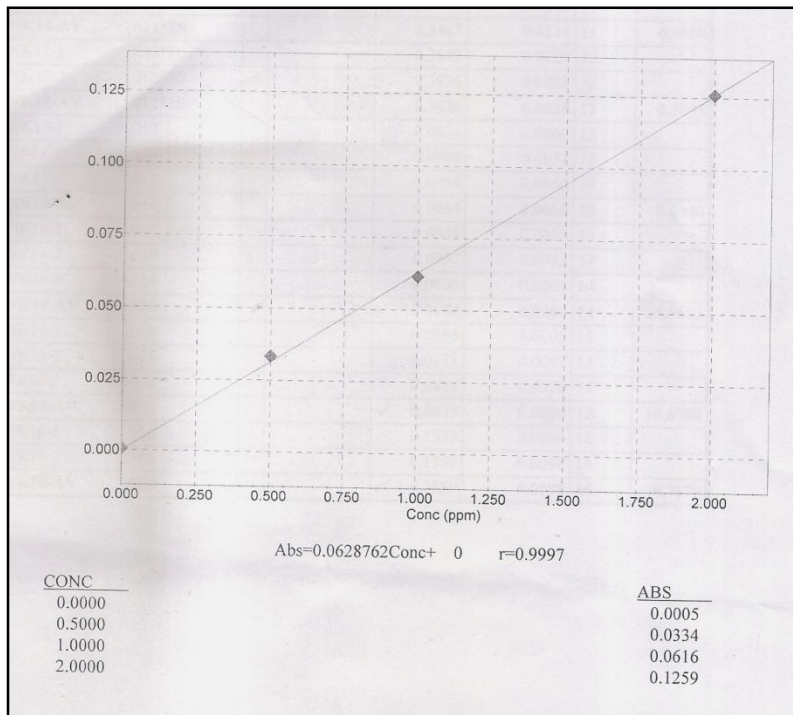
Fig 3.6: Calibration curve for the element iron (Fe)
