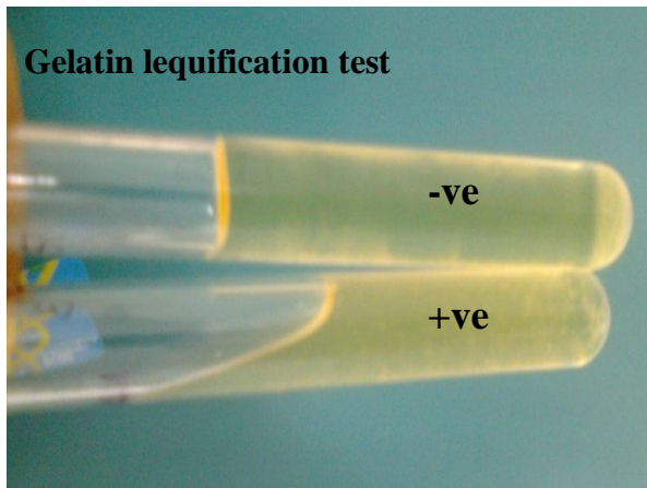
Plate 3.14: Gelatin liquefaction test
