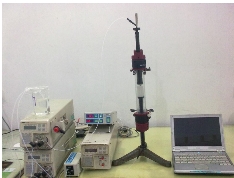
Figure 1-6: Operation of high performance liquid chromatography (HPLC).
