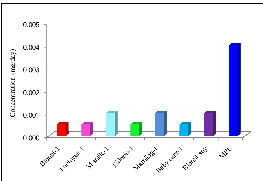
Figure 3.23: The comparison of concentration of cadmium in baby (0–6 months) powder milk of different brands with maximum permissible limit.
