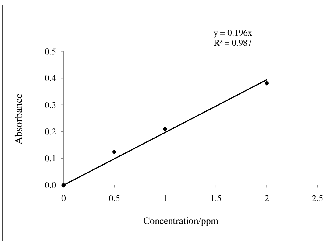
Figure 4.2: Calibration curve for the determination of potassium
