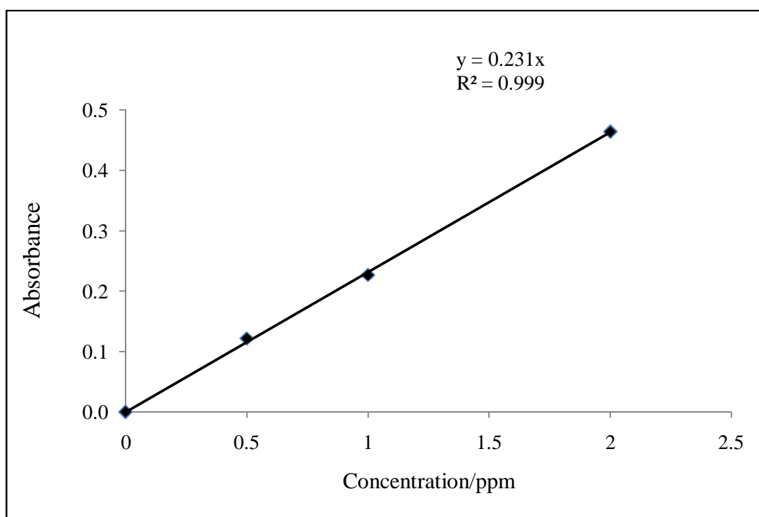
Figure 4.3: Calibration curve for the determination of calcium
