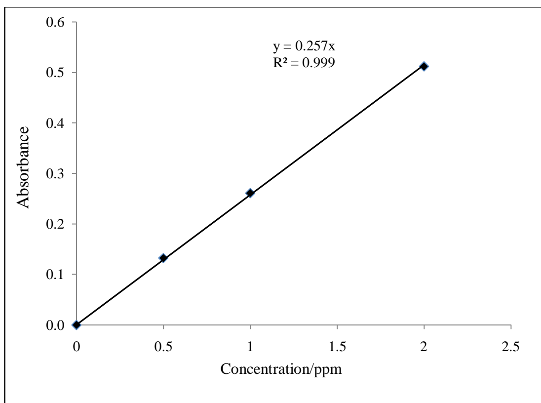
Figure 4.1: Calibration curve for the determination of sodium.
