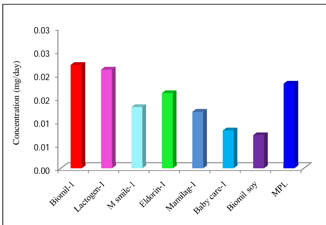
Figure 3.20: The variation of concentration of lead in baby (0–6 months) powder milk of different brands
