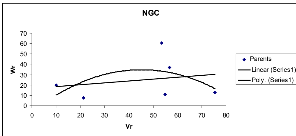
Graph 4. 2.10. Vr–Wr graph for number of grains/cob in 6x6 diallel cross in maize
