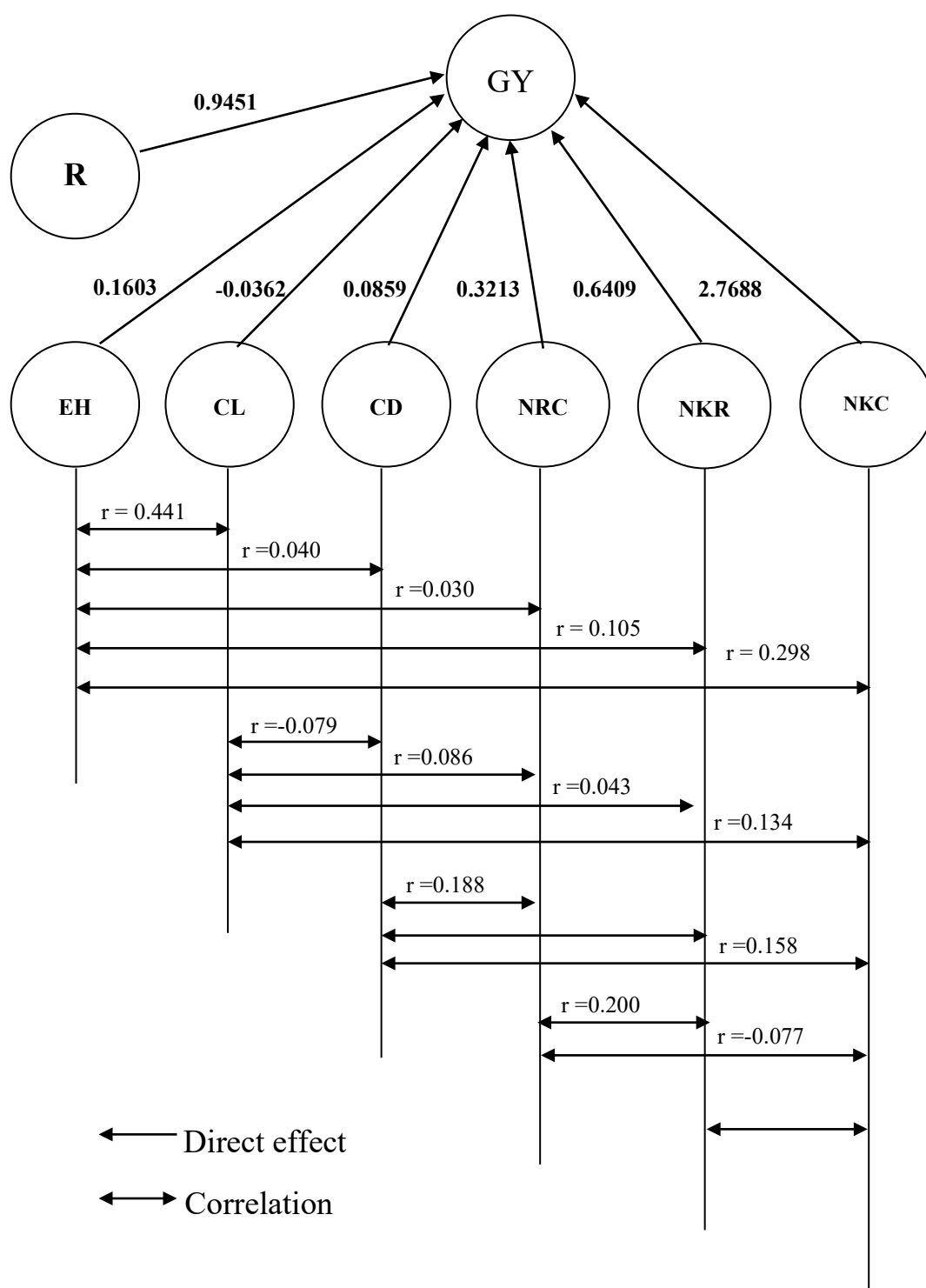
Figure 4.1.1. Path diagram of different grain yield contributing characters on yield at phenotypic level
