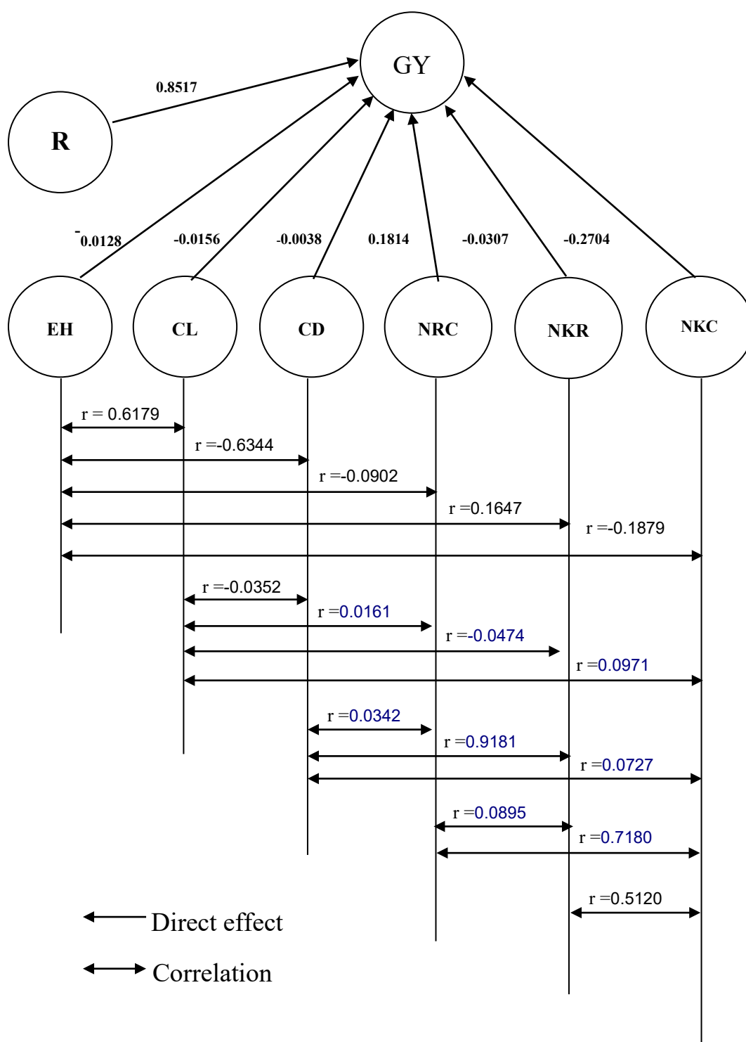
Figure 4.1.2. Path diagram of different grain yield contributing characters on yield at genotypic level
