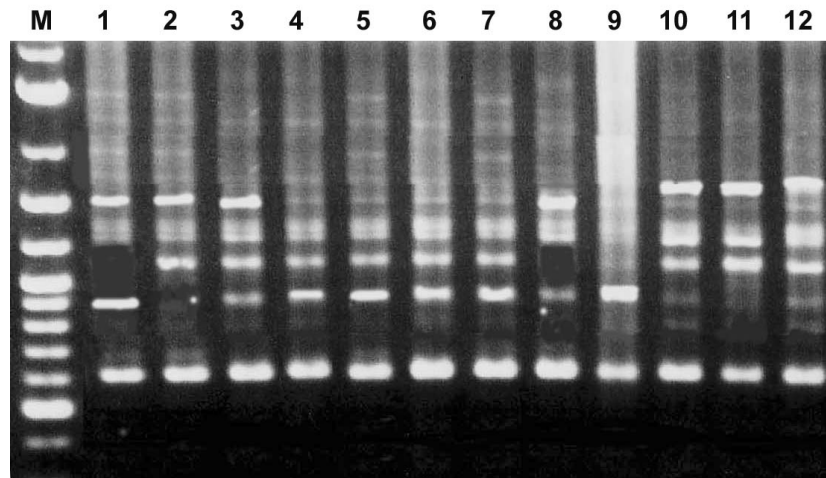
Figure 4.3 RAPD pattern amplified with primer OPA9 from the genomic DNA of tea genotypes. Lanes M= 1 kb size marker, 1= MZ/39, 2= E/4, 3= D/13, 4= B2xT1, 5= Br2/97, 6= SDL/1, 7= BT2, 8= Ph/9/4, 9= Ph/9/25, 10= Ph/9/40, 11= BS-67 and 12= BT5.
