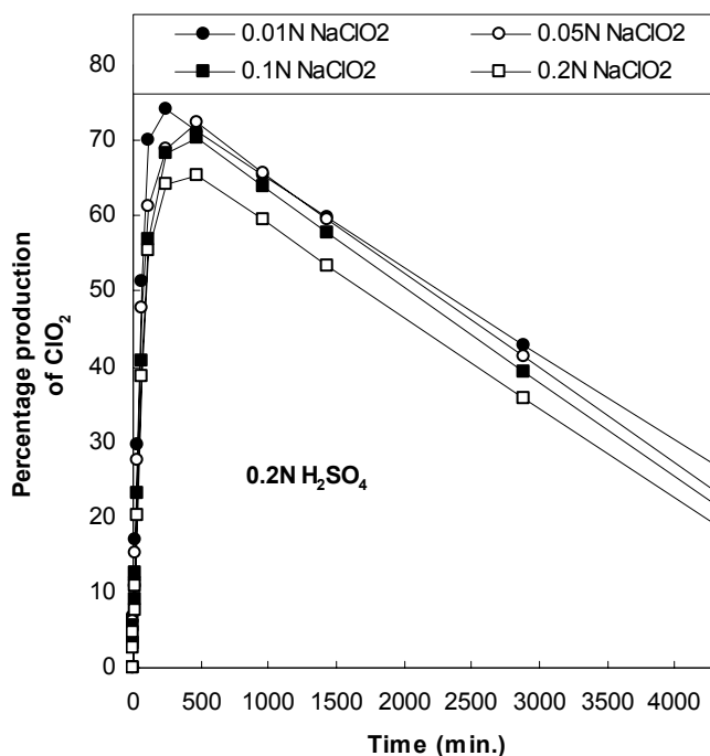
Fig. 5.15. The relation between the percentage productions of ClO 2 with time (min.) The reaction conditions: NaClO 2 : H 2 SO 4 (v/v) 1:1; at temperature 30 ± 1 o C [APPENDIX, Table-5.7.C for experimental data]
