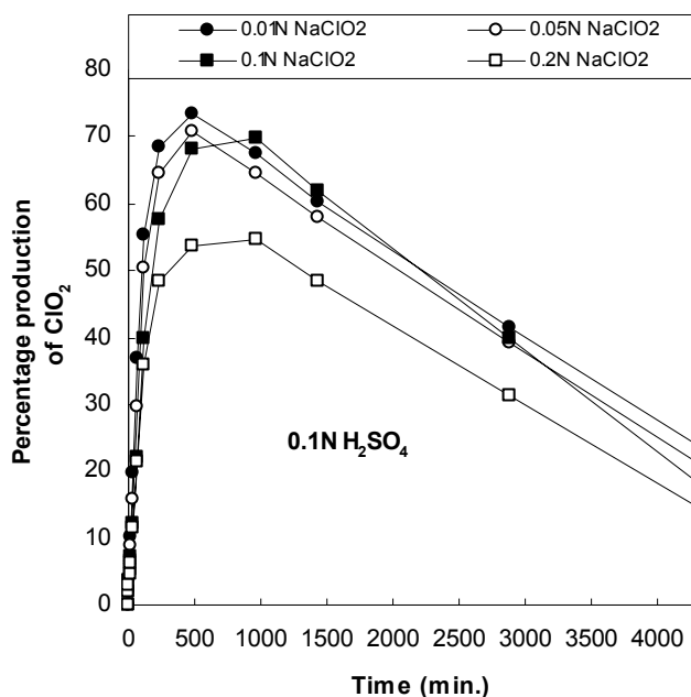
Fig. 5.14. The relation between the percentage productions of ClO 2 with time (min.) The reaction conditions: NaClO 2 : H 2 SO 4 (v/v) 1:1; at temperature 30 ± 1 o C [APPENDIX, Table-5.7.B for experimental data]
