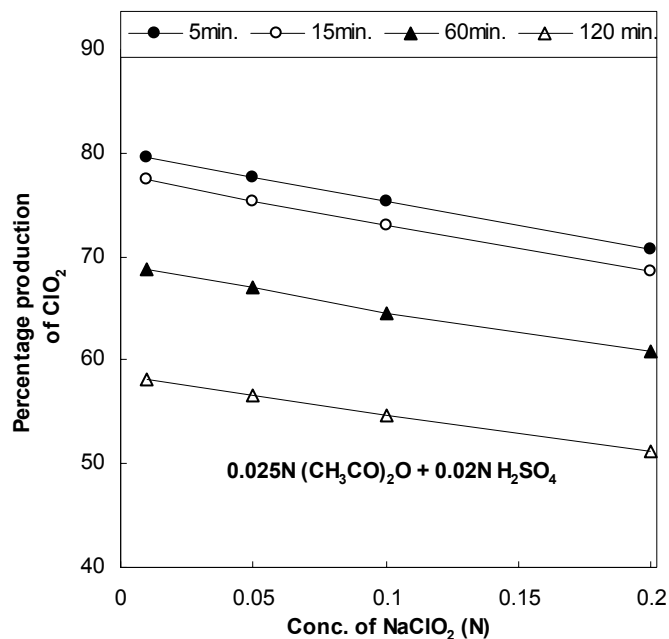
Fig. 5.53. The effect of NaClO 2 concentrations on the percentage production of ClO 2 Reaction conditions: NaClO 2 : (CH 3 CO) 2 O and H 2 SO 4 1: 1; at temperature, 30 ± 1 o C [APPENDIX, Table-5.25.A for experimental data]
