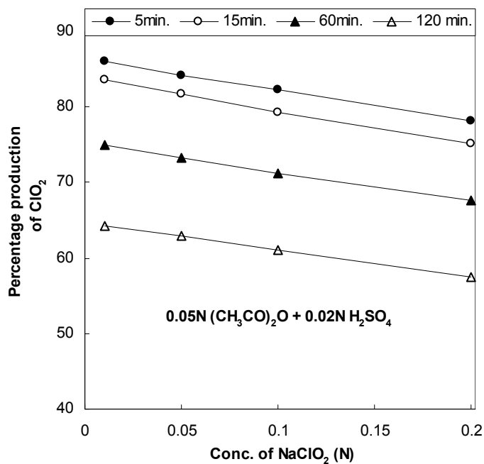
Fig. 5.54. The effect of NaClO 2 concentrations on the percentage production of ClO 2 Reaction conditions: NaClO 2 : (CH 3 CO) 2 O and H 2 SO 4 1: 1; at temperature, 30 ± 1 o C [APPENDIX, Table-5.25.B for experimental data]
