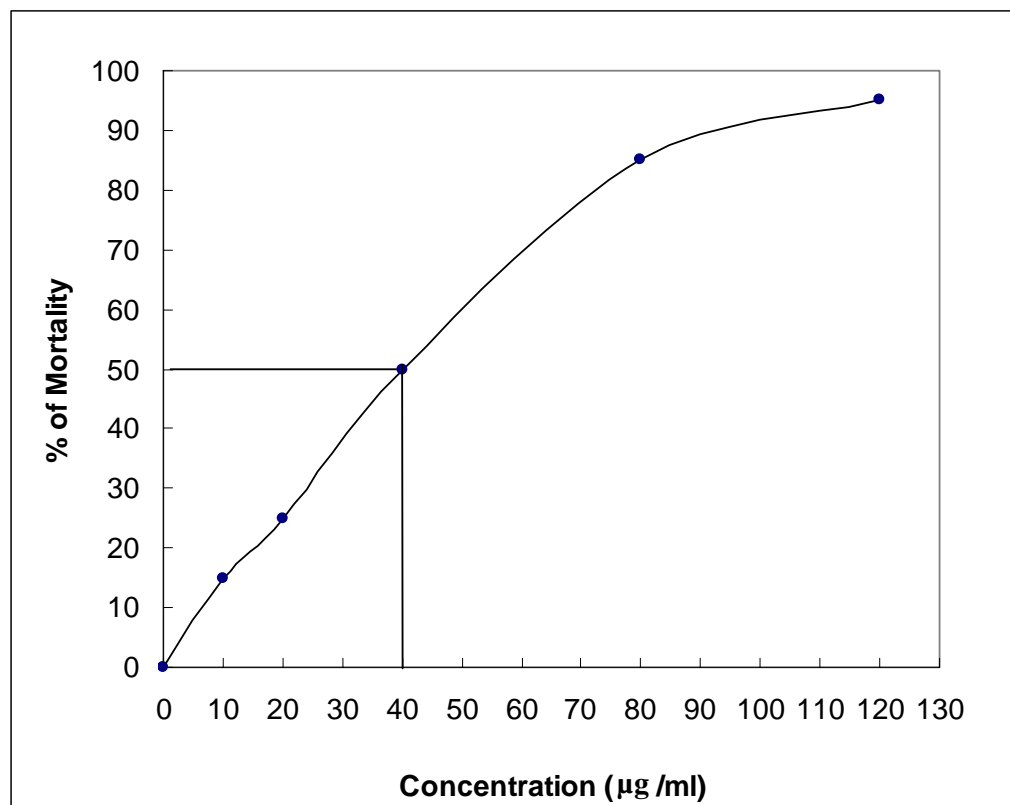
Fig-10: Determination of LC 50 of ethanol extract of the leaves of Vinca rosea L. against Brine Shrimp nauplii.
