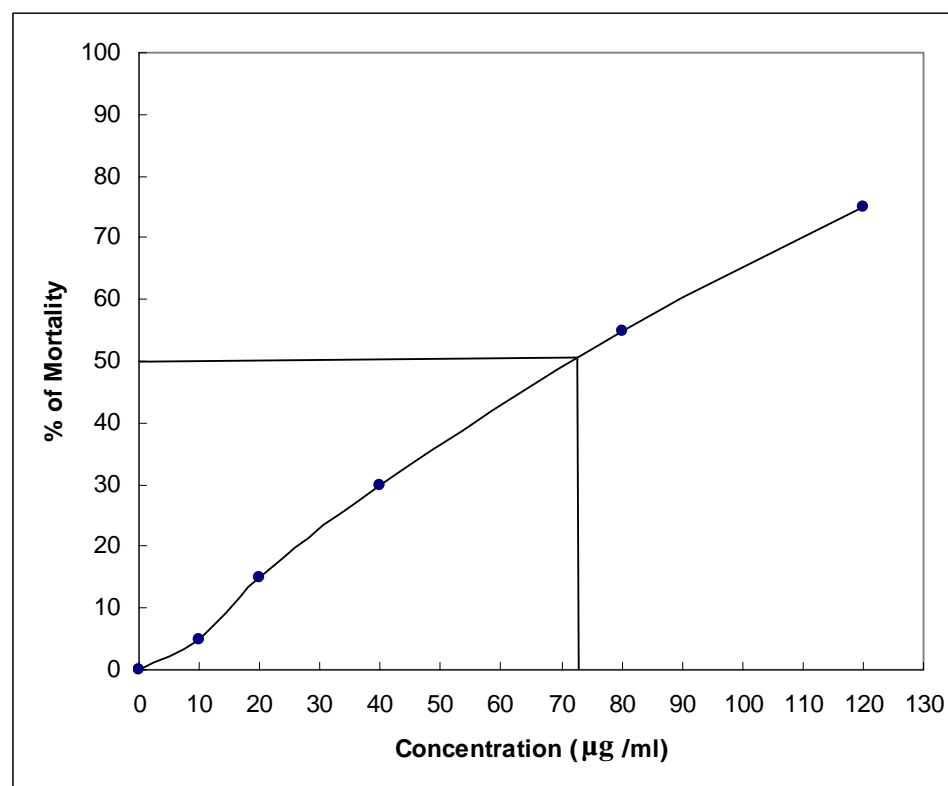
Fig-12: Determination of \text{LC}_{50} of ethanol extract of the leaves of Vitex vegundo L. against Brine Shrimp nauplii.
