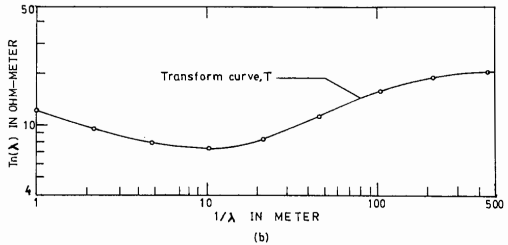
Fig. 3.4 Derivation of the resistivity transform from the sampled values of the apparent resistivity field curve. (a) sampling of e_a curve (b) resultant T curve, of the example of Figure-3.3
