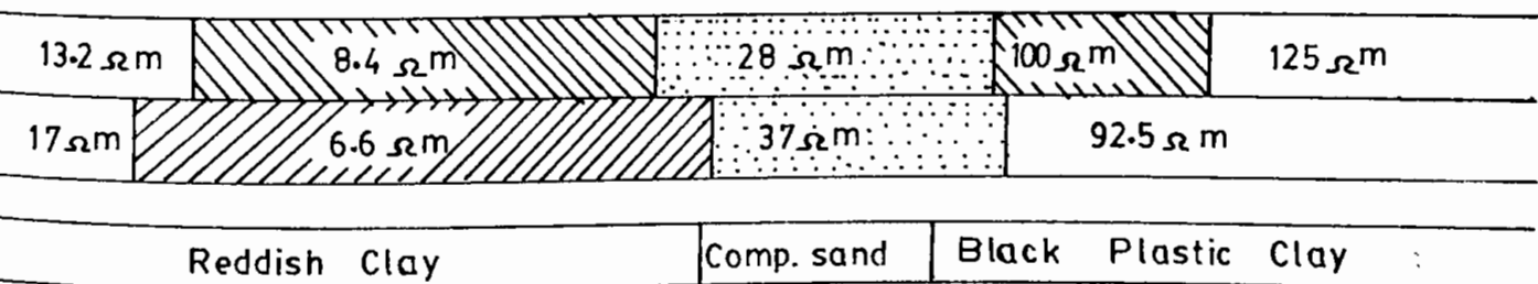
Fig.4.4 Interpreted field curves of VES-4; (a) March 1991, (b) June 1992.
