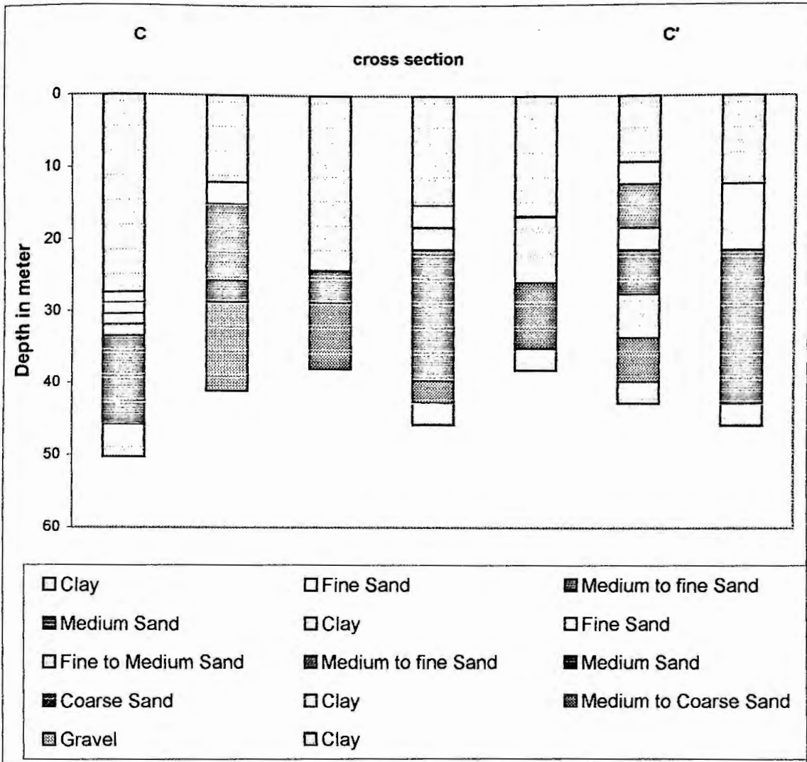
Fig. 4.8: Hydrogeological cross-section along CC'.
